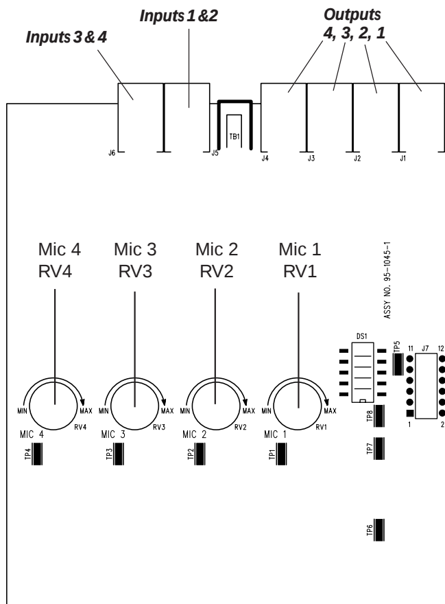
95-1045-1 Mic Preamp Card
